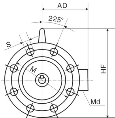
YE3-225~280
